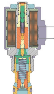
Cartridge valve cutaway
